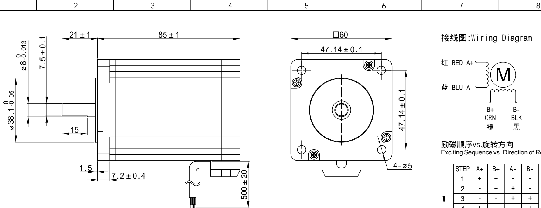
从安装面看为顺时针方向 Clockwise view from mouting side
